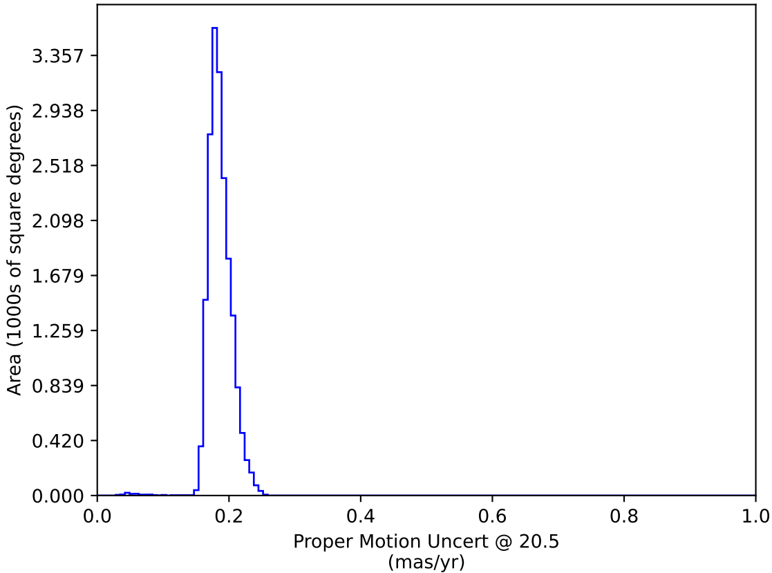
ddf_loaded_fl4_v3.4_10yrs WFD: Proper Motion Uncert @ 20.5
