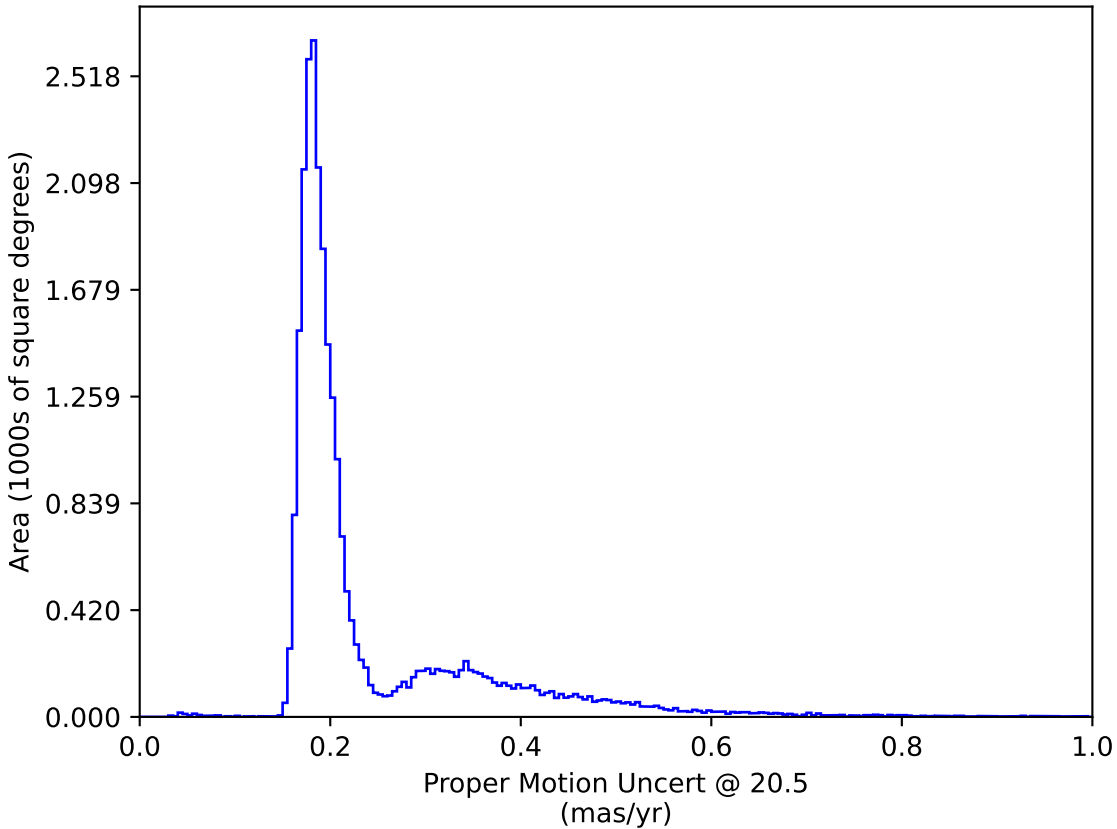
ddf_loaded_fl4_v3.4_10yrs All sky: Proper Motion Uncert @ 20.5
