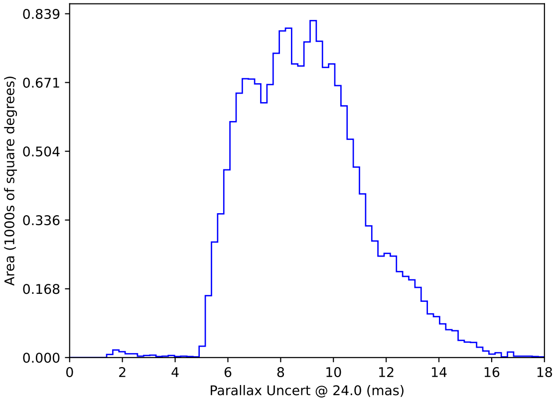
ddf_loaded_fl4_v3.4_10yrs WFD: Parallax Uncert @ 24.0
