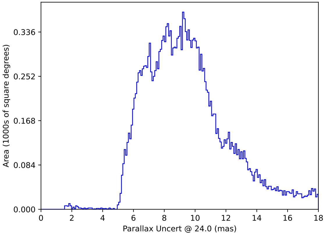
ddf_loaded_fl4_v3.4_10yrs All sky: Parallax Uncert @ 24.0
