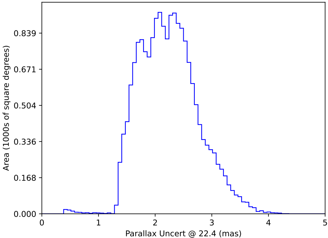
ddf_loaded_fl4_v3.4_10yrs WFD: Parallax Uncert @ 22.4
