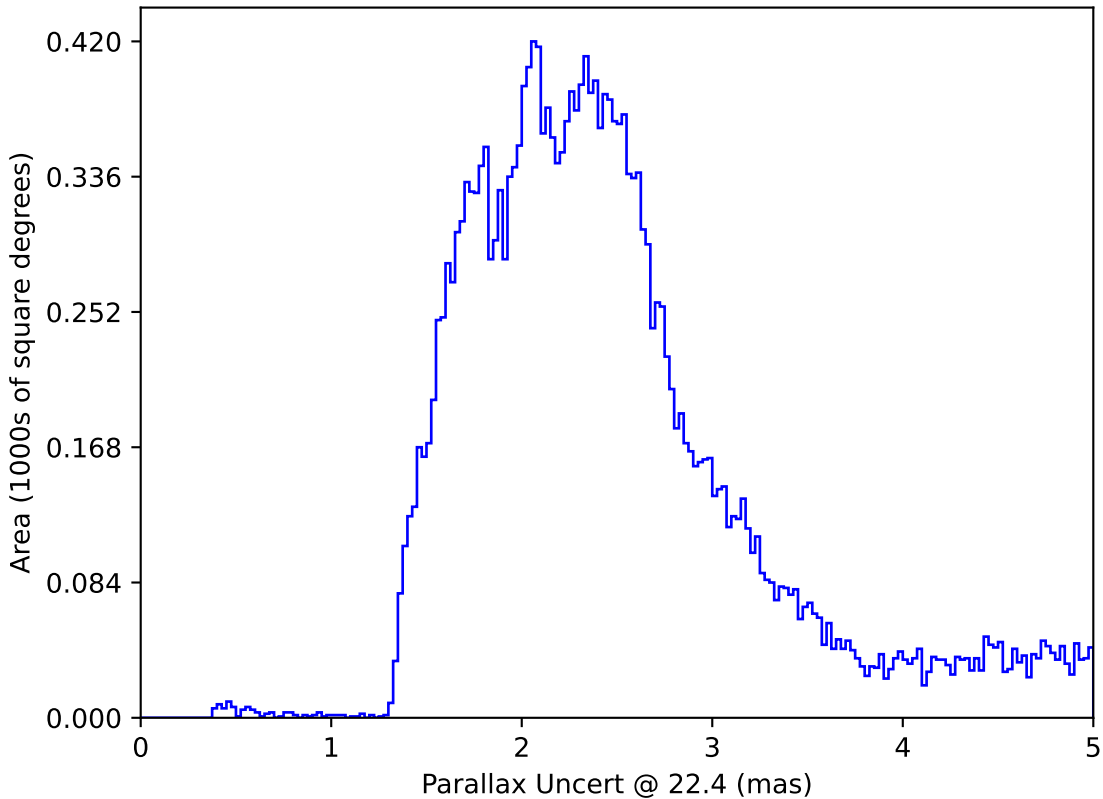
ddf_loaded_fl4_v3.4_10yrs All sky: Parallax Uncert @ 22.4
