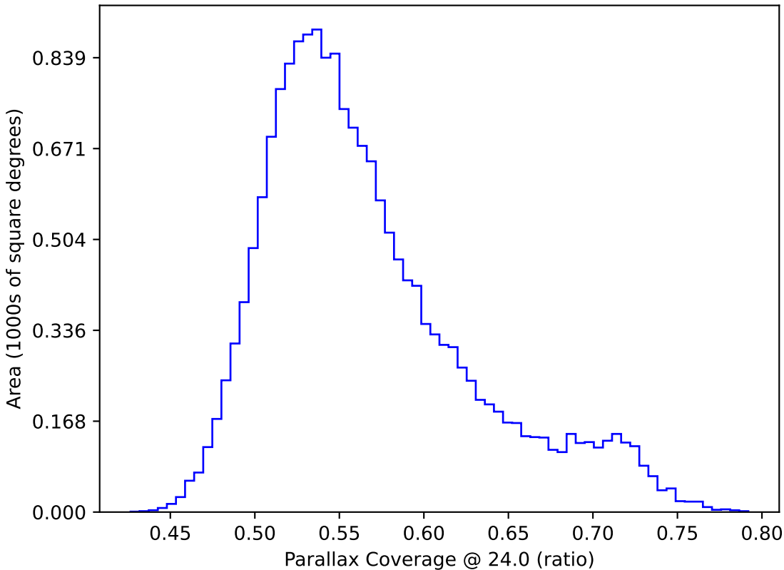
ddf_loaded_fl4_v3.4_10yrs WFD: Parallax Coverage @ 24.0
