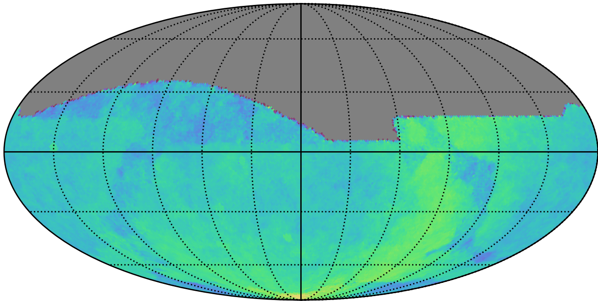
ddf_loaded_fl4_v3.4_10yrs All sky: Parallax Coverage @ 24.0
