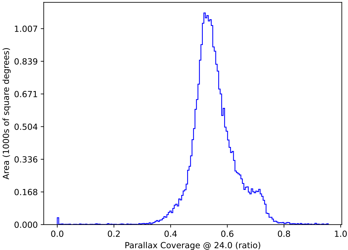
ddf_loaded_fl4_v3.4_10yrs All sky: Parallax Coverage @ 24.0
