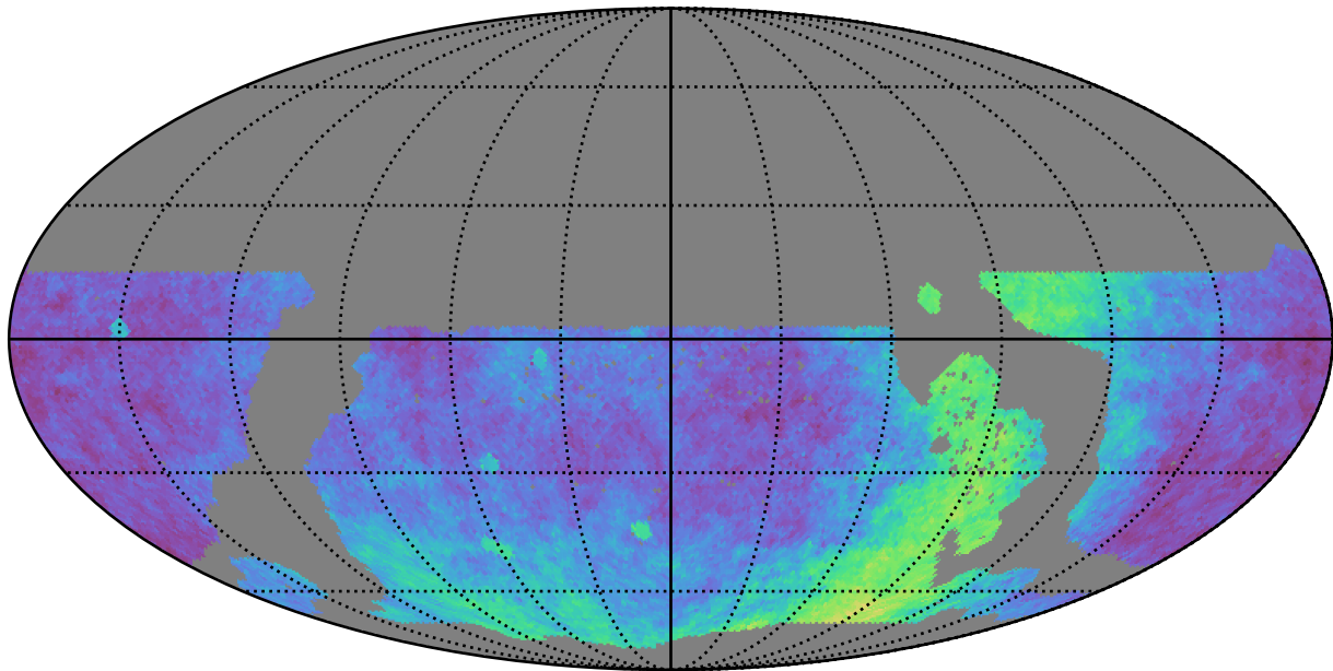
ddf_loaded_fl4_v3.4_10yrs WFD: Parallax Coverage @ 22.4
