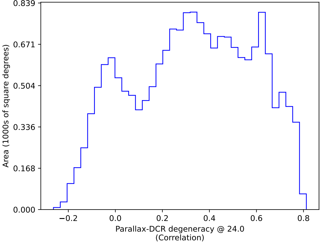
ddf_loaded_fl4_v3.4_10yrs WFD: Parallax-DCR degeneracy @ 24.0
