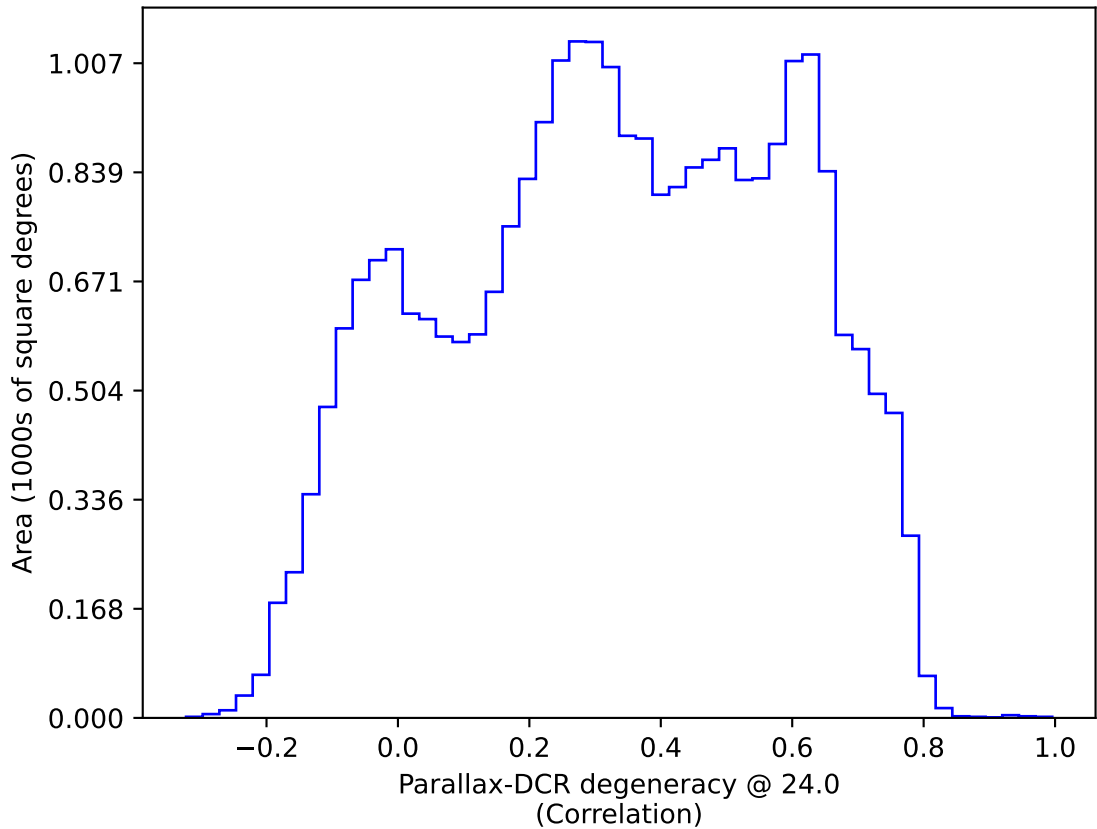
ddf_loaded_fl4_v3.4_10yrs All sky: Parallax-DCR degeneracy @ 24.0
