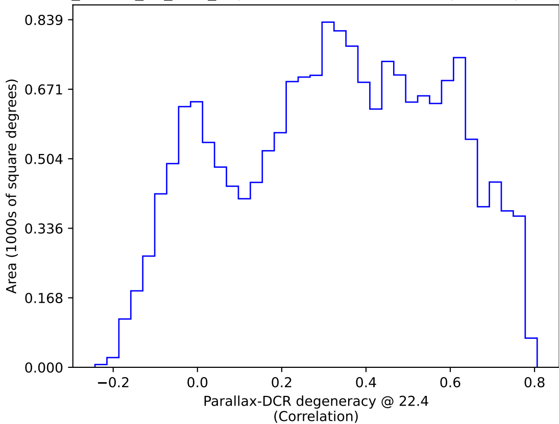
ddf_loaded_fl4_v3.4_10yrs WFD: Parallax-DCR degeneracy @ 22.4
