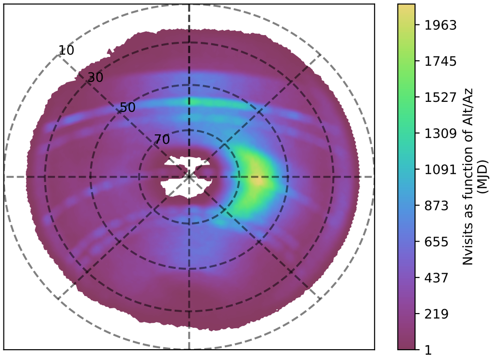
ddf_loaded_fl4_v3.4_10yrs z band: Nvisits as function of Alt/Az
