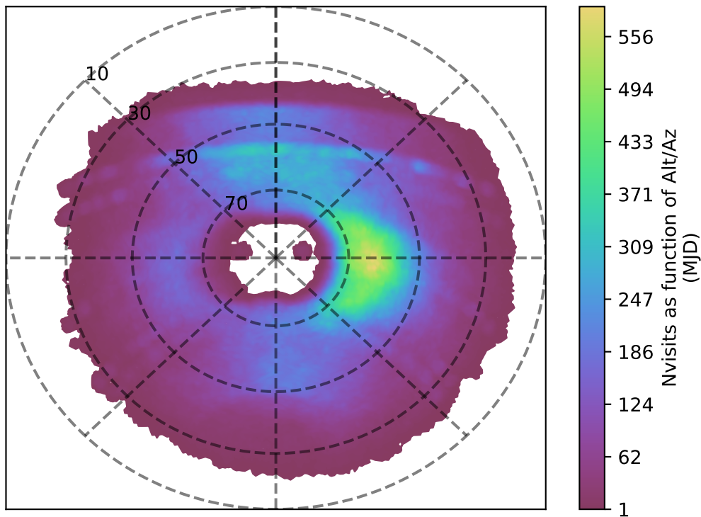
ddf_loaded_fl4_v3.4_10yrs u band: Nvisits as function of Alt/Az
