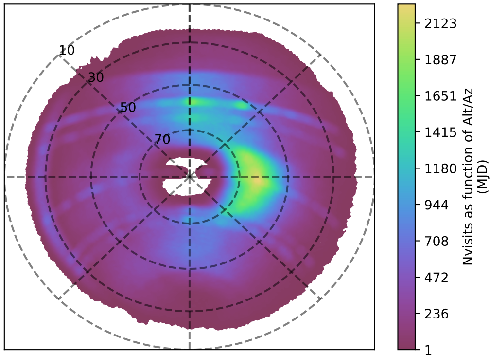
ddf_loaded_fl4_v3.4_10yrs r band: Nvisits as function of Alt/Az
