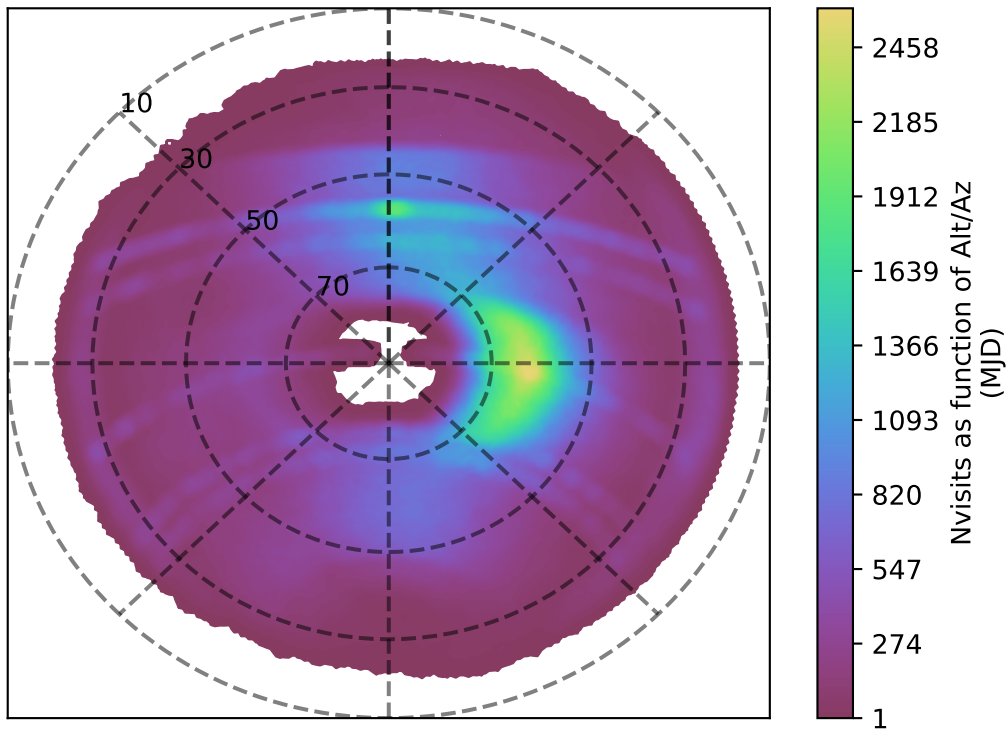
ddf_loaded_fl4_v3.4_10yrs i band: Nvisits as function of Alt/Az
