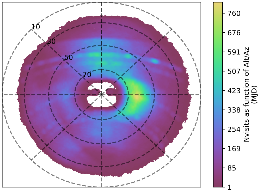
ddf_loaded_fl4_v3.4_10yrs g band: Nvisits as function of Alt/Az
