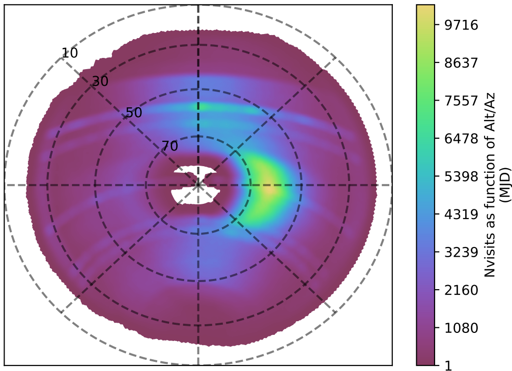
ddf_loaded_fl4_v3.4_10yrs all bands: Nvisits as function of Alt/Az
