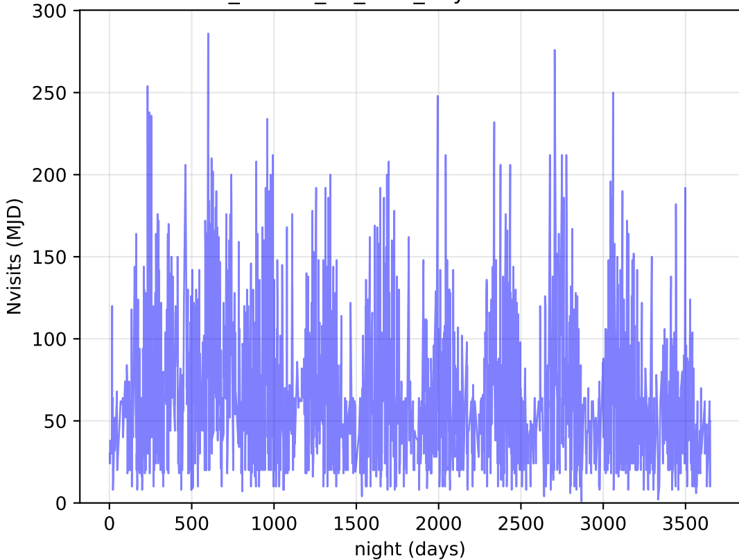
ddf_loaded_fl4_v3.4_10yrs DDF: Nvisits
