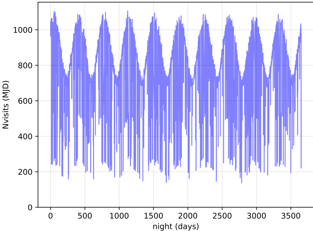
ddf_loaded_fl4_v3.4_10yrs All visits: Nvisits
