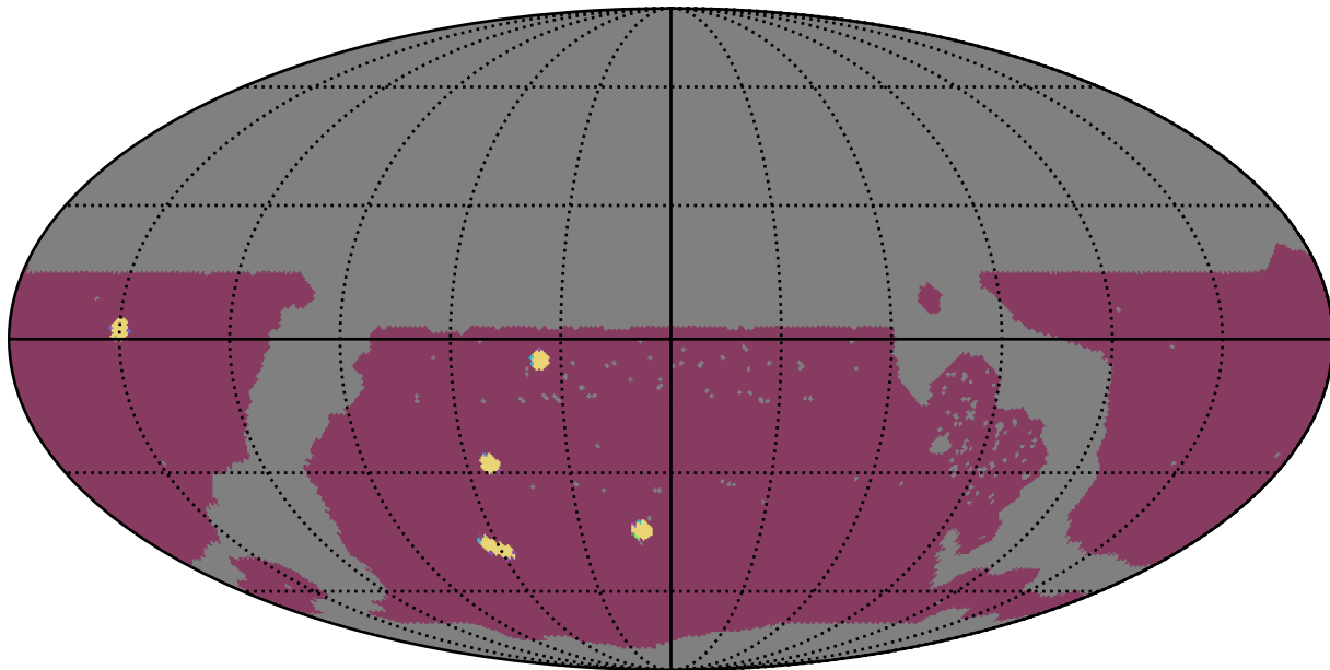
ddf_loaded_fl4_v3.4_10yrs WFD: NumberOfQuickRevisits
