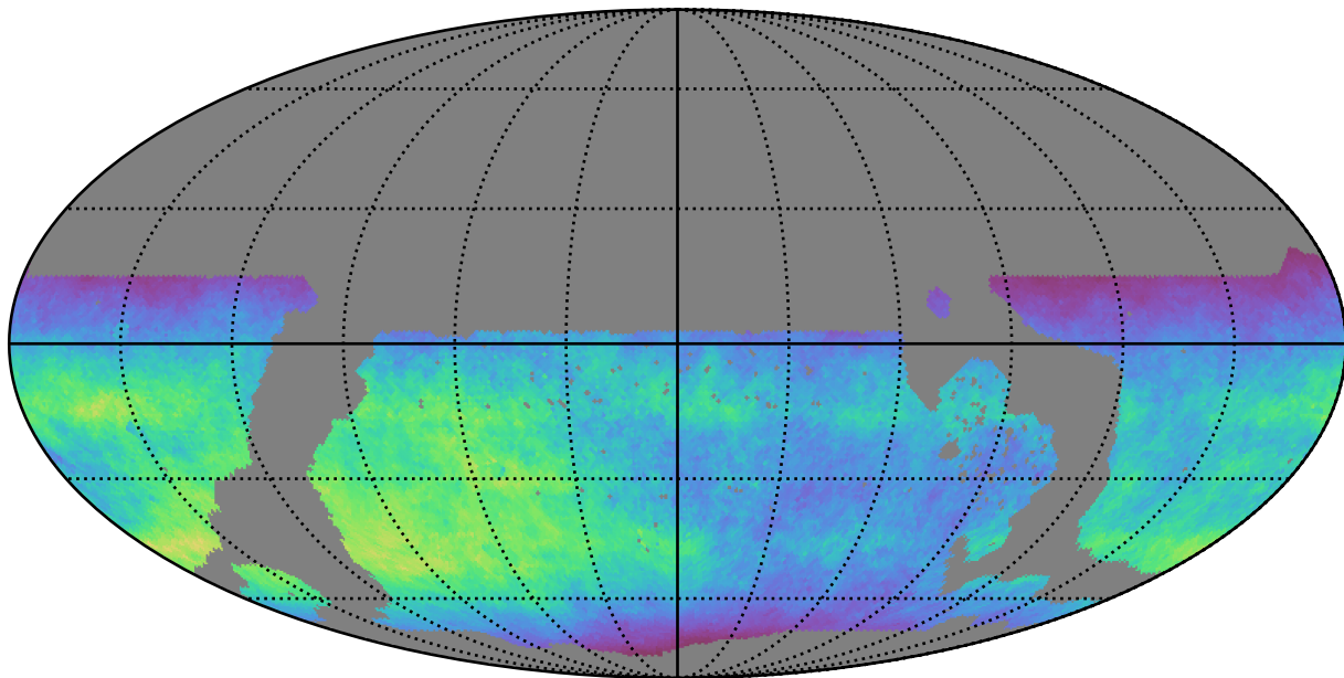
ddf_loaded_fl4_v3.4_10yrs WFD z band: Normalized Teff
