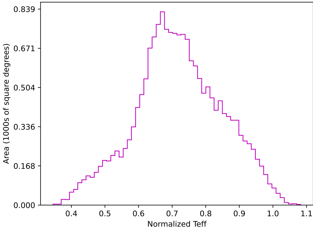
ddf_loaded_fl4_v3.4_10yrs WFD z band: Normalized Teff
