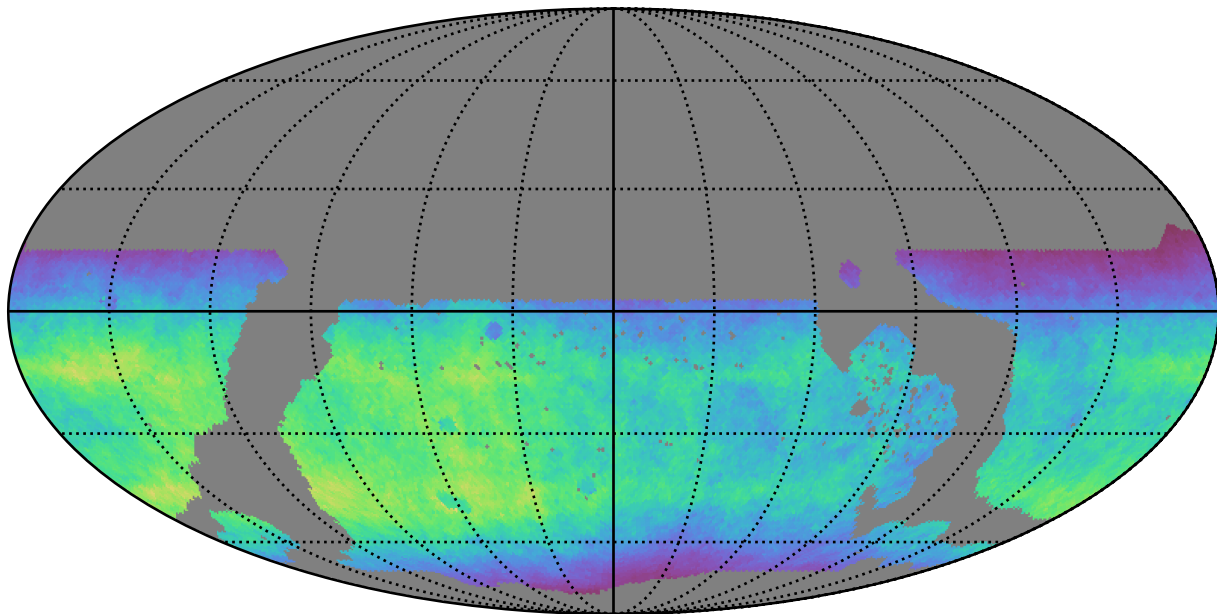
ddf_loaded_fl4_v3.4_10yrs WFD y band: Normalized Teff
