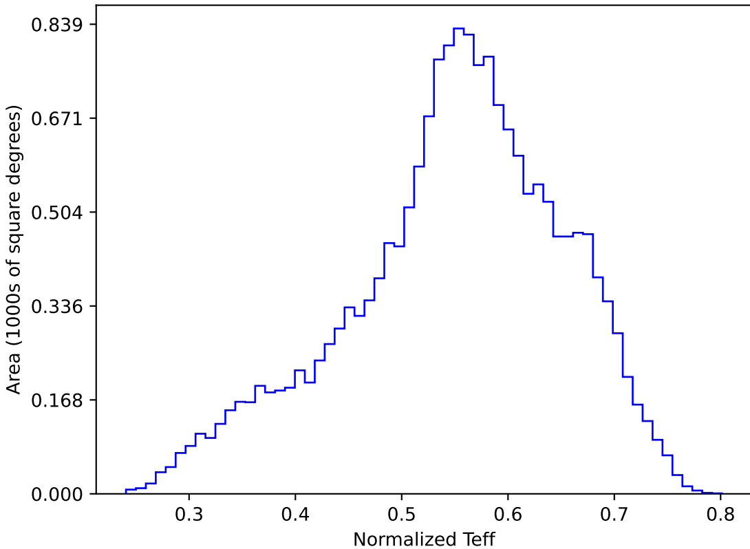
ddf_loaded_fl4_v3.4_10yrs WFD y band: Normalized Teff
