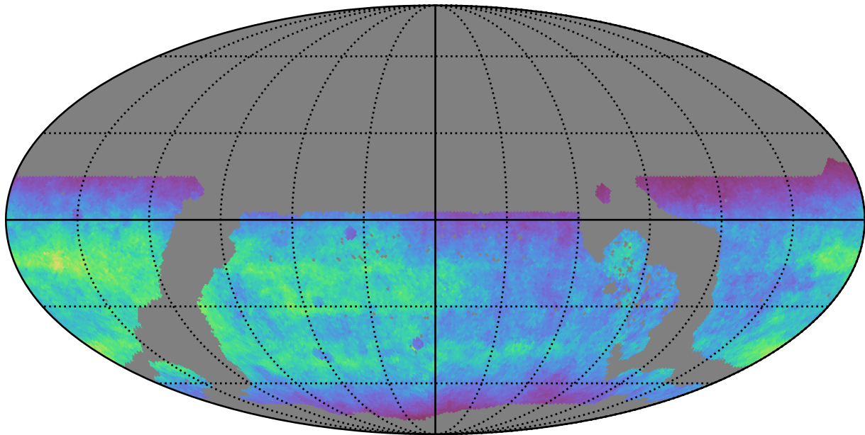
ddf_loaded_fl4_v3.4_10yrs WFD u band: Normalized Teff
