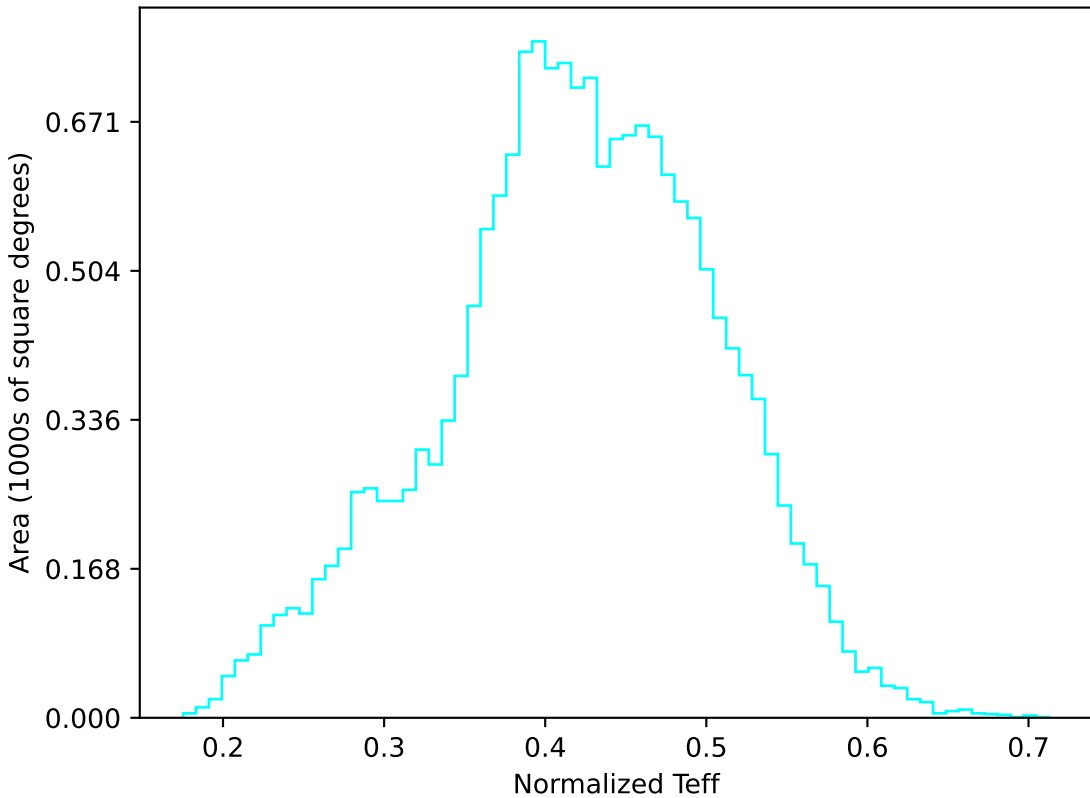
ddf_loaded_fl4_v3.4_10yrs WFD u band: Normalized Teff
