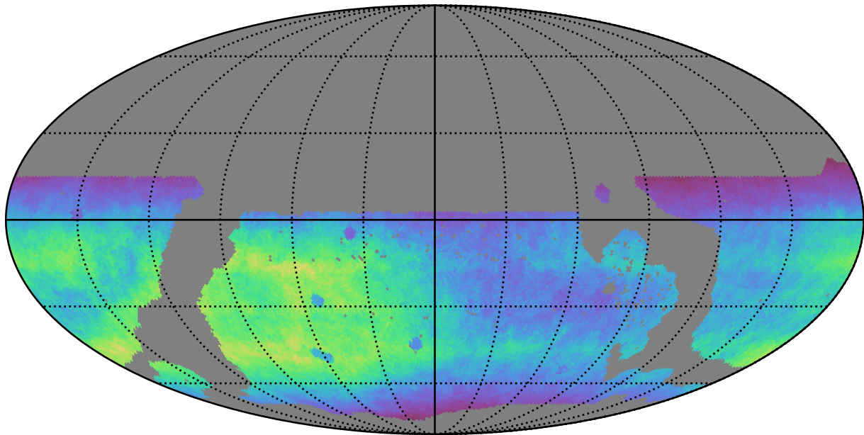
ddf_loaded_fl4_v3.4_10yrs WFD r band: Normalized Teff
