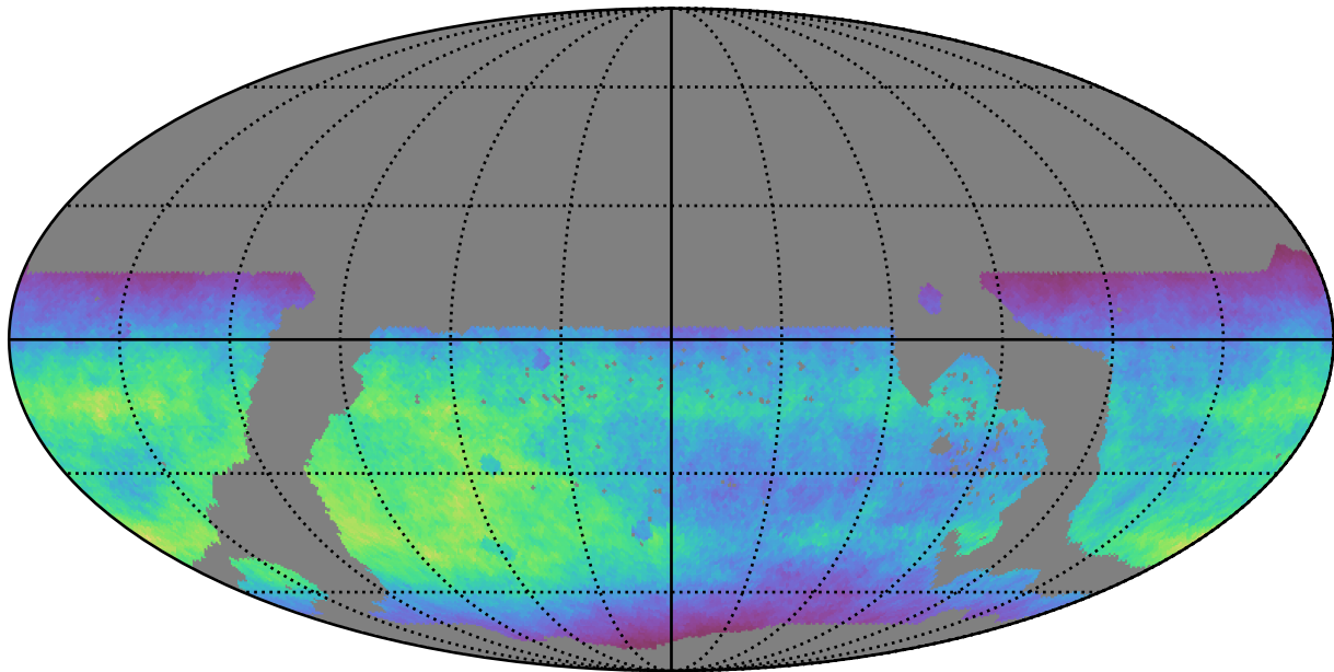
ddf_loaded_fl4_v3.4_10yrs WFD i band: Normalized Teff
