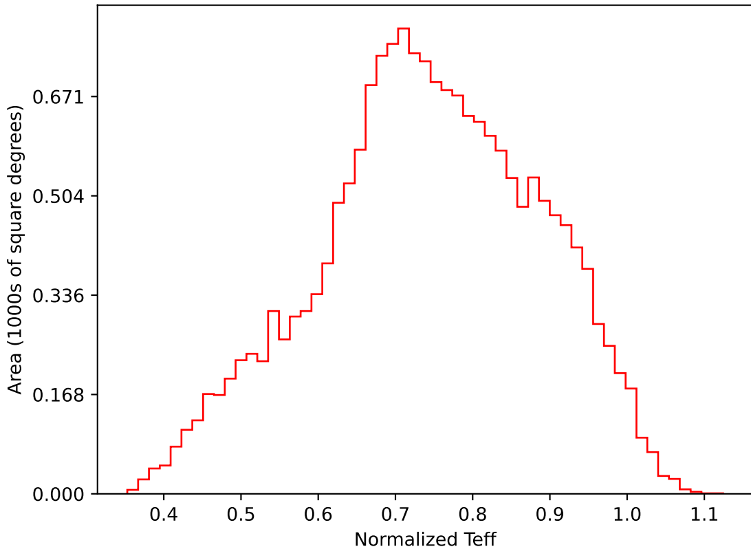
ddf_loaded_fl4_v3.4_10yrs WFD i band: Normalized Teff
