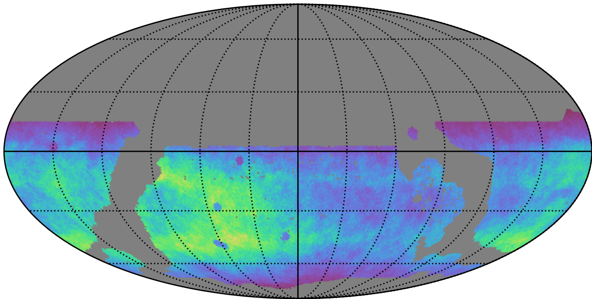
ddf_loaded_fl4_v3.4_10yrs WFD g band: Normalized Teff
