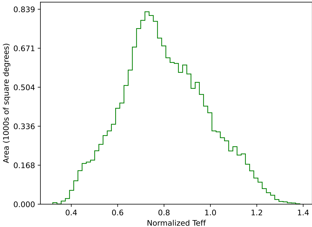
ddf_loaded_fl4_v3.4_10yrs WFD g band: Normalized Teff
