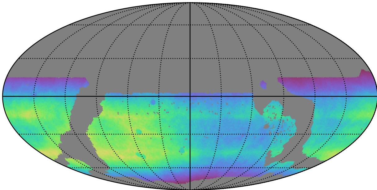
ddf_loaded_fl4_v3.4_10yrs WFD all bands: Normalized Teff
