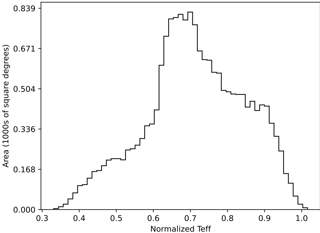
ddf_loaded_fl4_v3.4_10yrs WFD all bands: Normalized Teff
