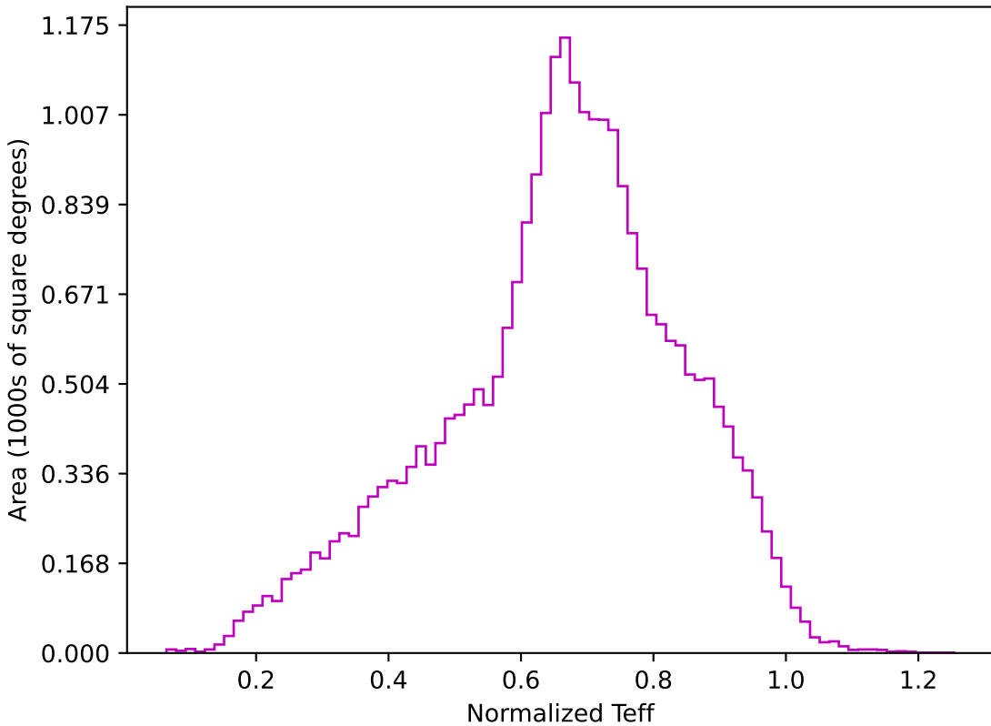
ddf_loaded_fl4_v3.4_10yrs All sky z band: Normalized Teff
