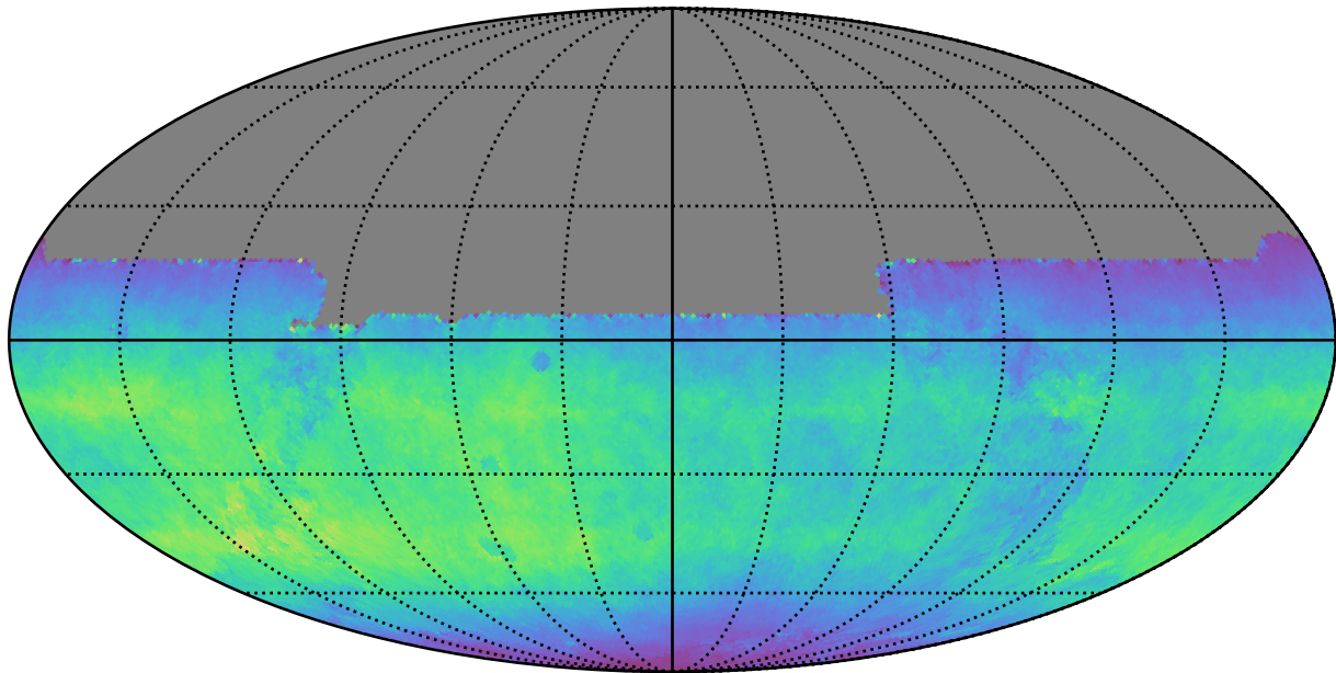
ddf_loaded_fl4_v3.4_10yrs All sky y band: Normalized Teff
