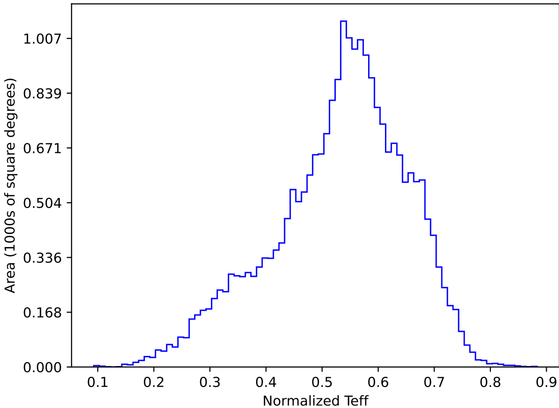
ddf_loaded_fl4_v3.4_10yrs All sky y band: Normalized Teff
