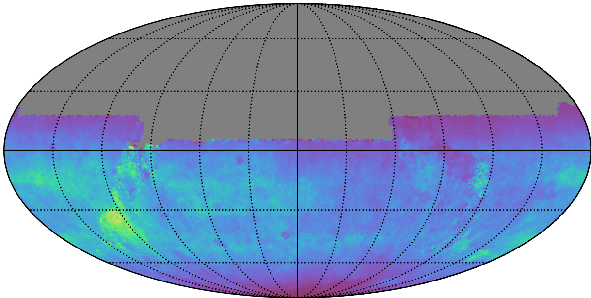
ddf_loaded_fl4_v3.4_10yrs All sky u band: Normalized Teff
