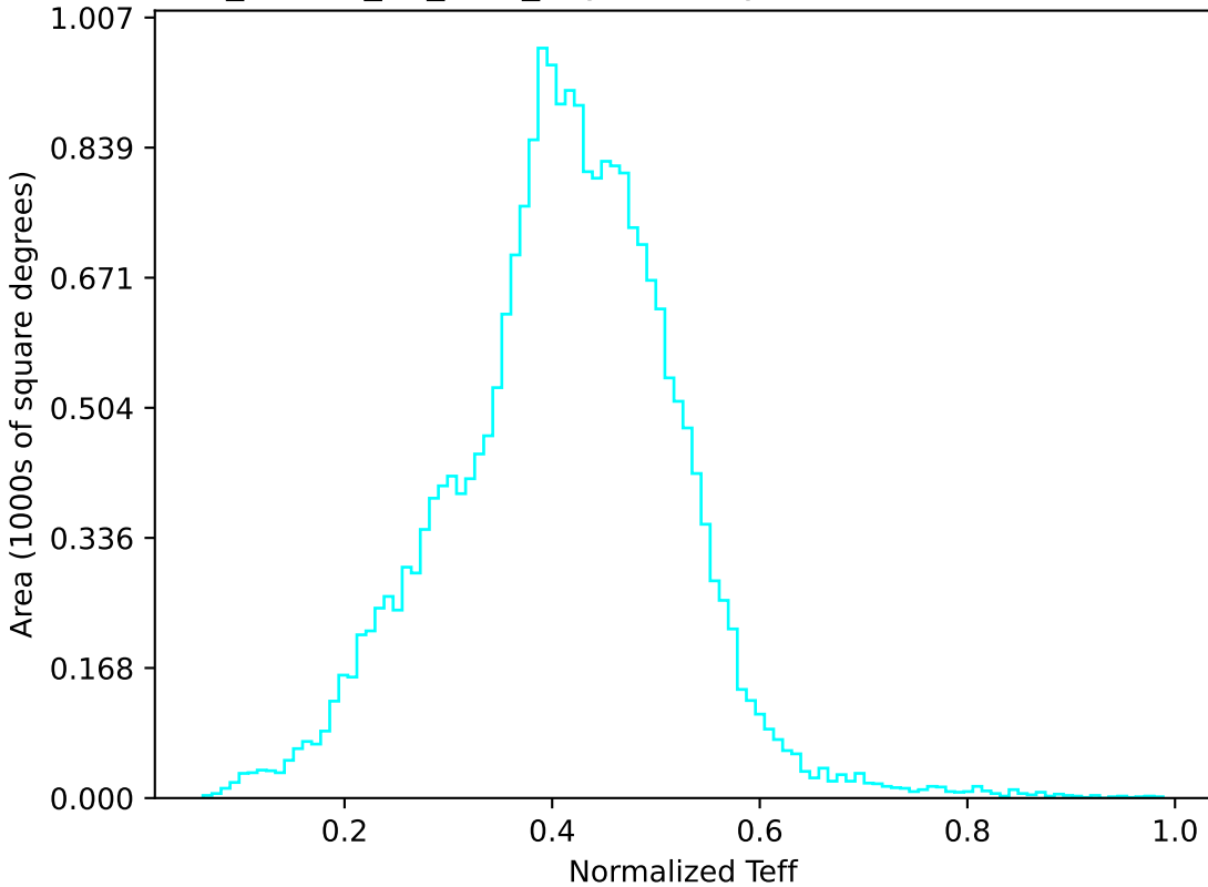
ddf_loaded_fl4_v3.4_10yrs All sky u band: Normalized Teff
