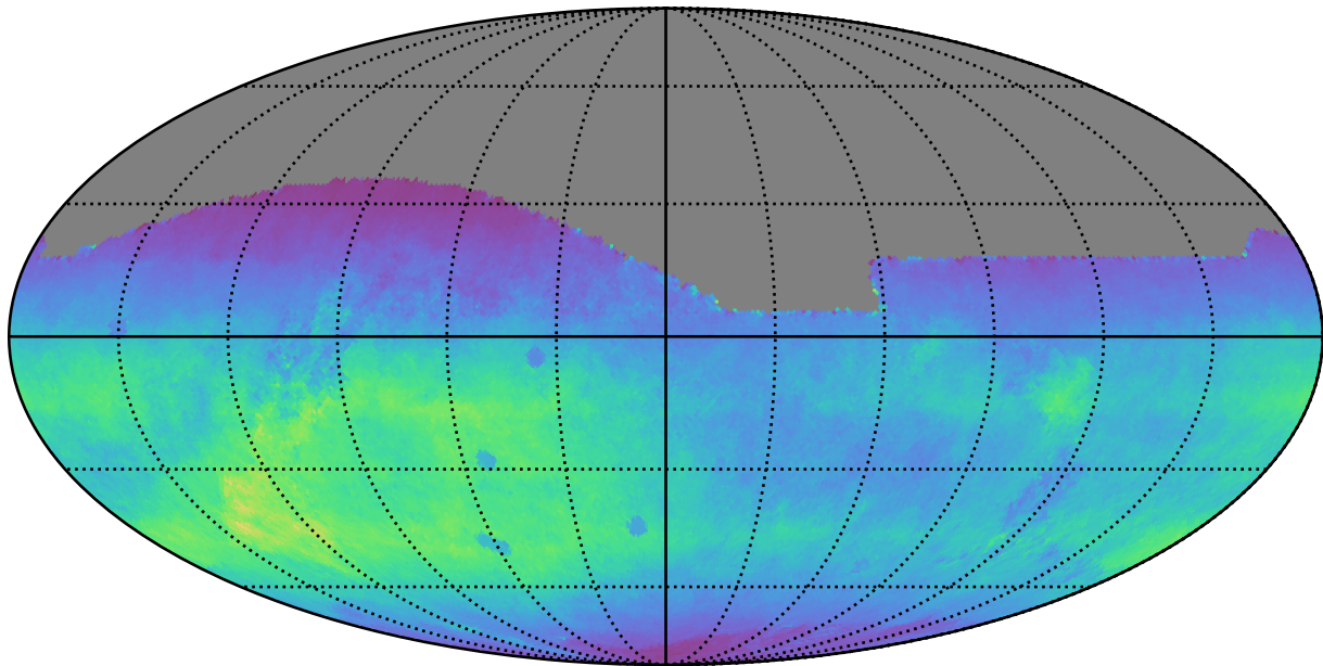
ddf_loaded_fl4_v3.4_10yrs All sky r band: Normalized Teff
