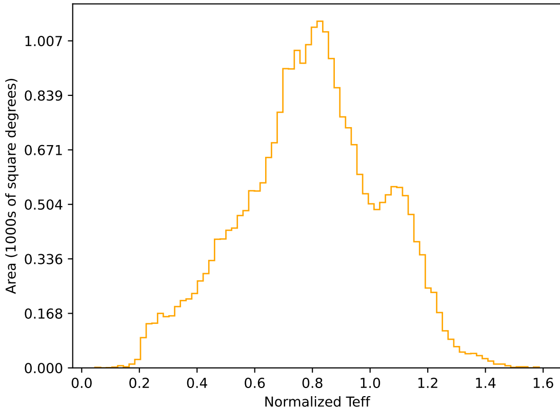
ddf_loaded_fl4_v3.4_10yrs All sky r band: Normalized Teff
