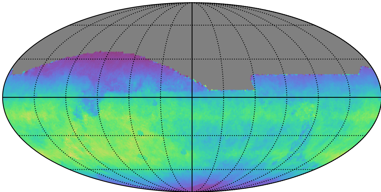
ddf_loaded_fl4_v3.4_10yrs All sky i band: Normalized Teff
