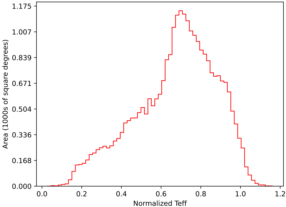
ddf_loaded_fl4_v3.4_10yrs All sky i band: Normalized Teff
