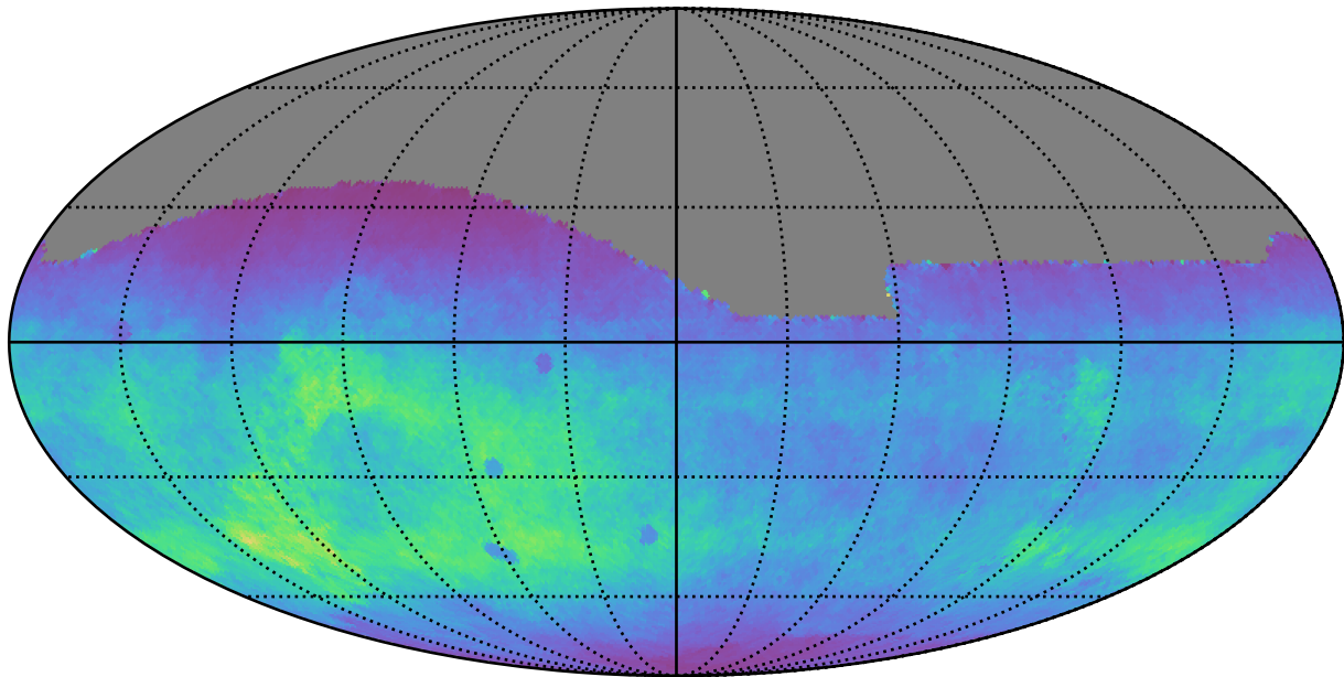
ddf_loaded_fl4_v3.4_10yrs All sky g band: Normalized Teff
