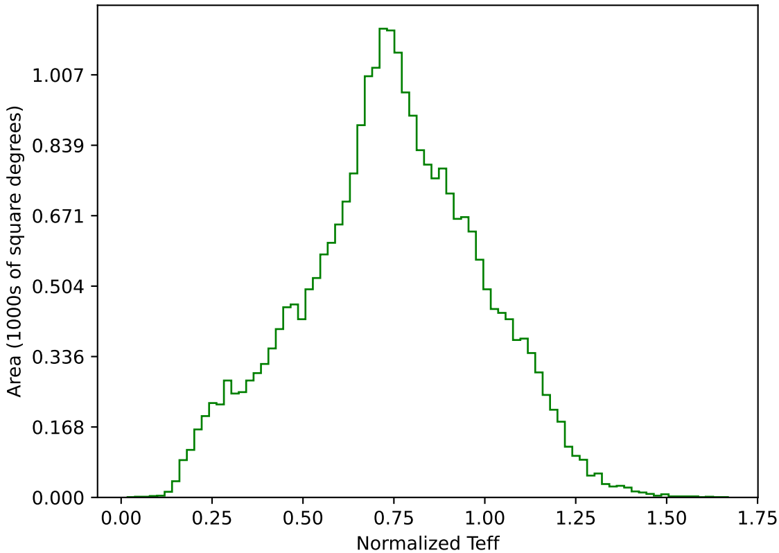
ddf_loaded_fl4_v3.4_10yrs All sky g band: Normalized Teff
