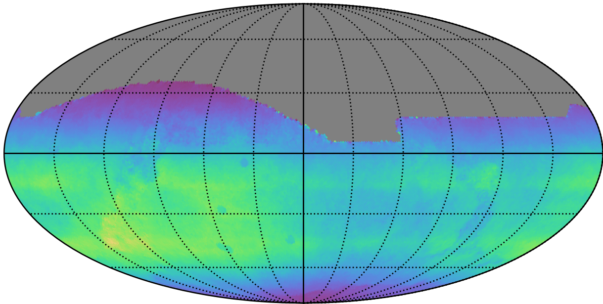
ddf_loaded_fl4_v3.4_10yrs All sky all bands: Normalized Teff
