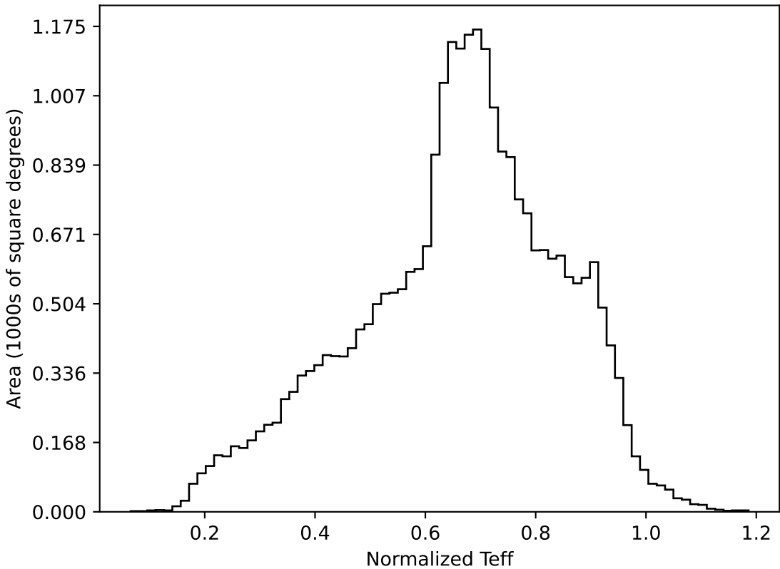
ddf_loaded_fl4_v3.4_10yrs All sky all bands: Normalized Teff
