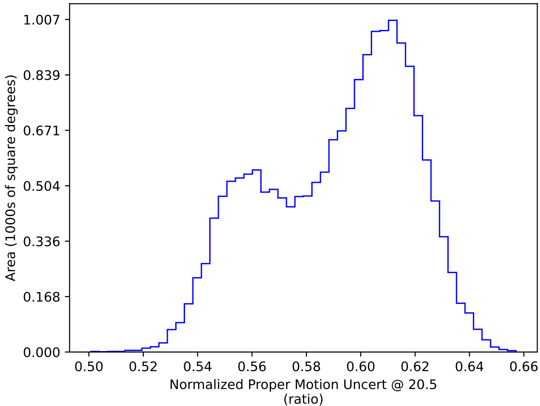
ddf_loaded_fl4_v3.4_10yrs WFD: Normalized Proper Motion Uncert @ 20.5
