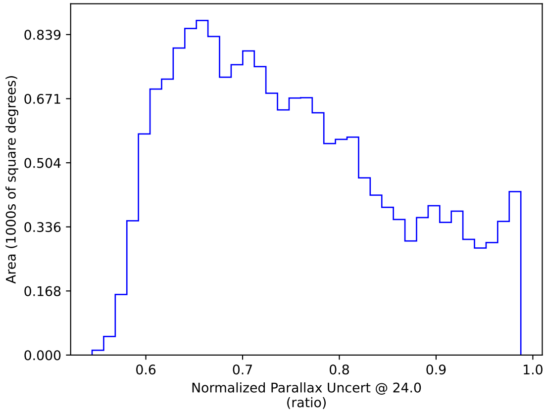
ddf_loaded_fl4_v3.4_10yrs WFD: Normalized Parallax Uncert @ 24.0
